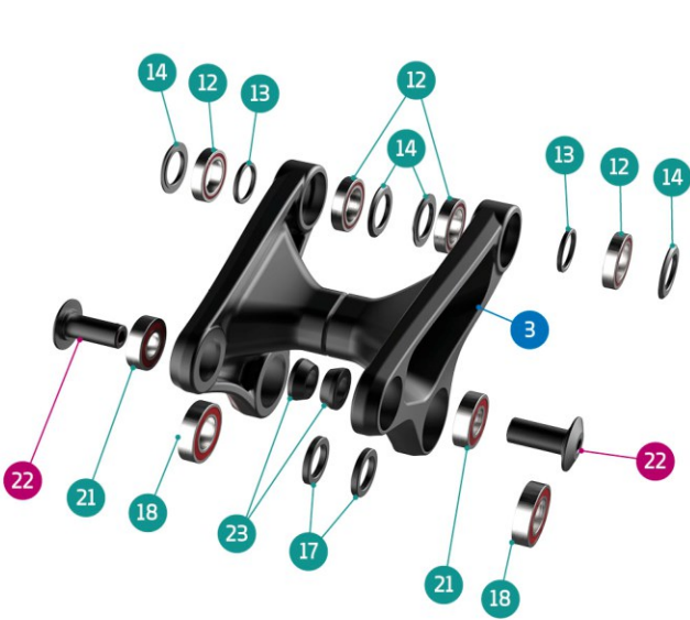
DETAIL 01
